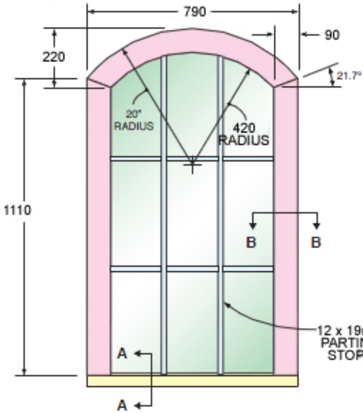
Shop-Made Window
