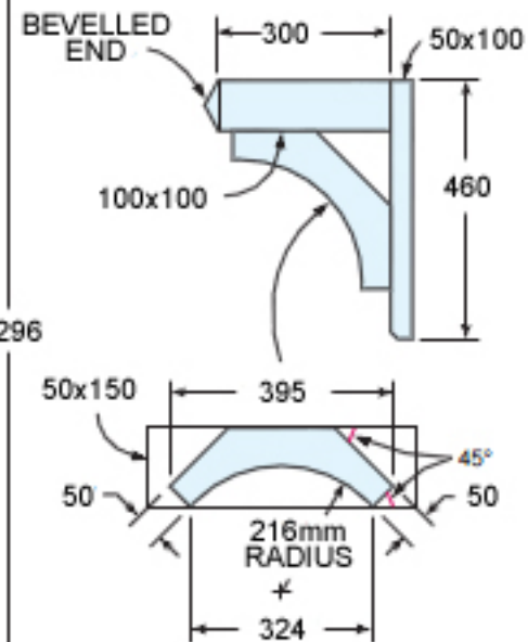
Shop-Made Bracket
