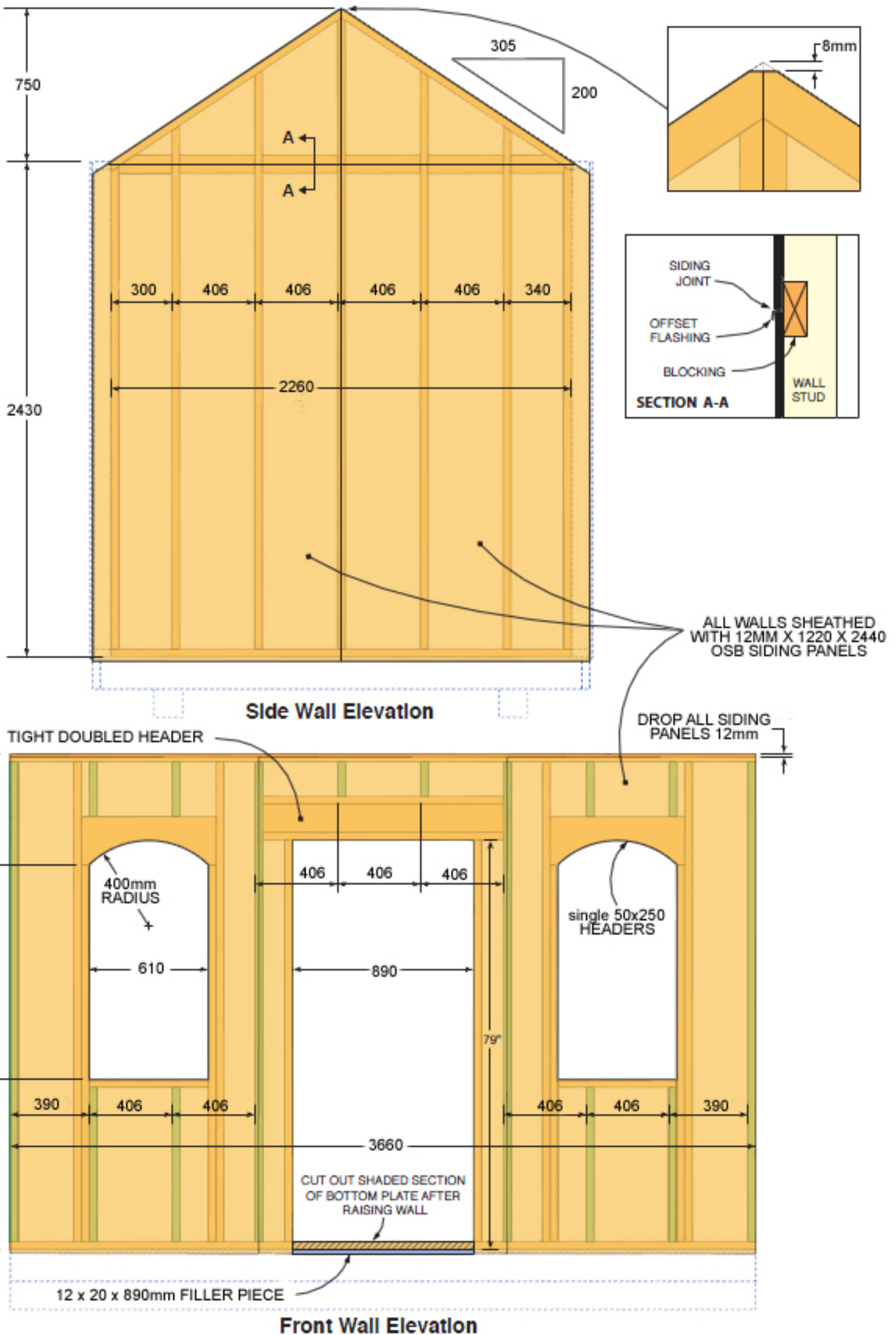
Figure C Wall framing
